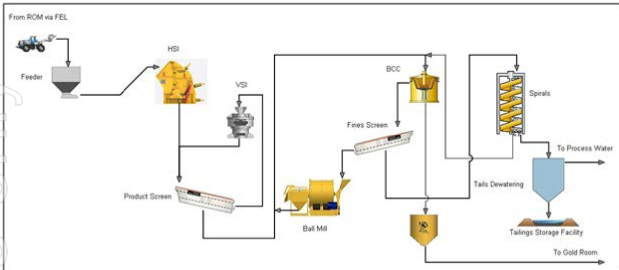
Figure 7 – Processing Flowsheet
