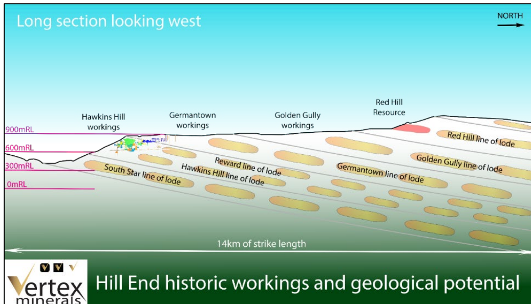
Figure 2 - Line of Lode from Hawkins Hill to Red Hill (Note the limited shallow historical mining along the 14km strike)
