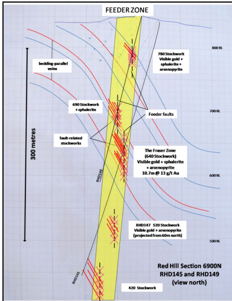
Figure 4 - Red Hill stockwork zones
