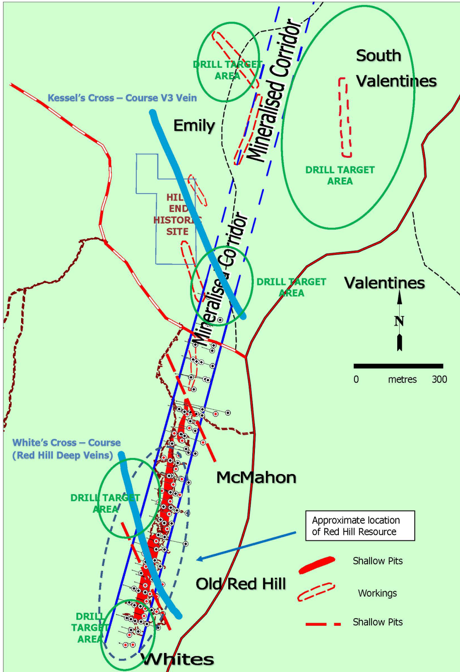
Figure 3 Locations of proposed drilling at Red Hill (outlined in green)
